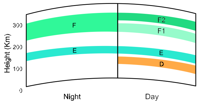
Ionospheric layers
