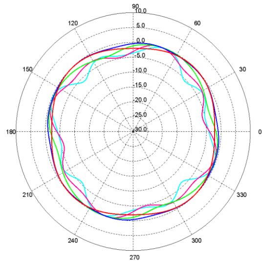
Normalised Azimuth (E-Plane) Pattern for Band B
